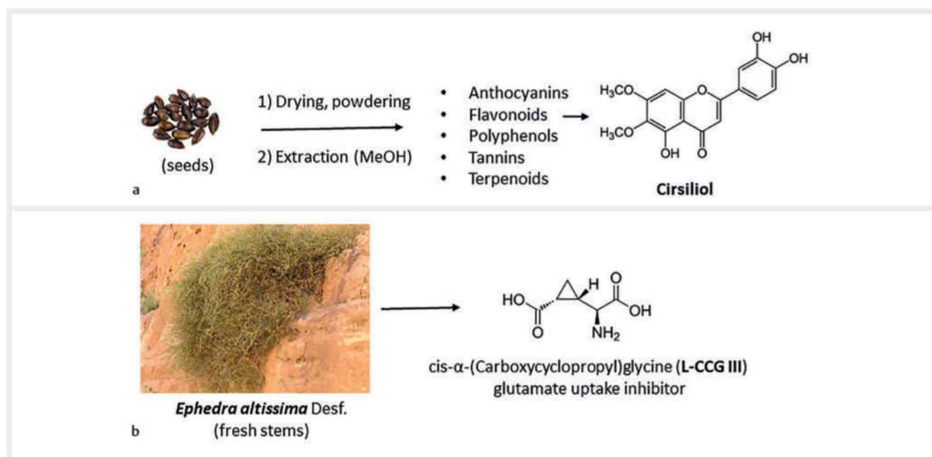
► Fig. 4 E. altissima with the extraction process used to extract various natural products from the seeds, including the flavonoid cirsiol or the glutamate uptake inhibitor L-CCG III (cis- \alpha -(carboxycyclopropyl) glycine) from the fresh stems of the plant (photo of the plant from https://www.teline.fr ; photo credit: Jean-Claude Thiaudière).
